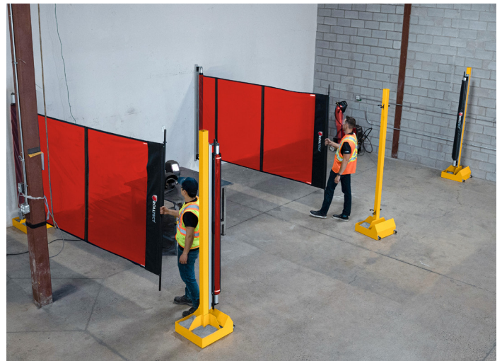
WHEN WELDING OPERATIONS ARE READY, THE OPERATOR WILL TAKE CONTROL OF THE CURTAIN AND HOOK IT TO THE J-HOOK ON THE OPPOSITE POST.
