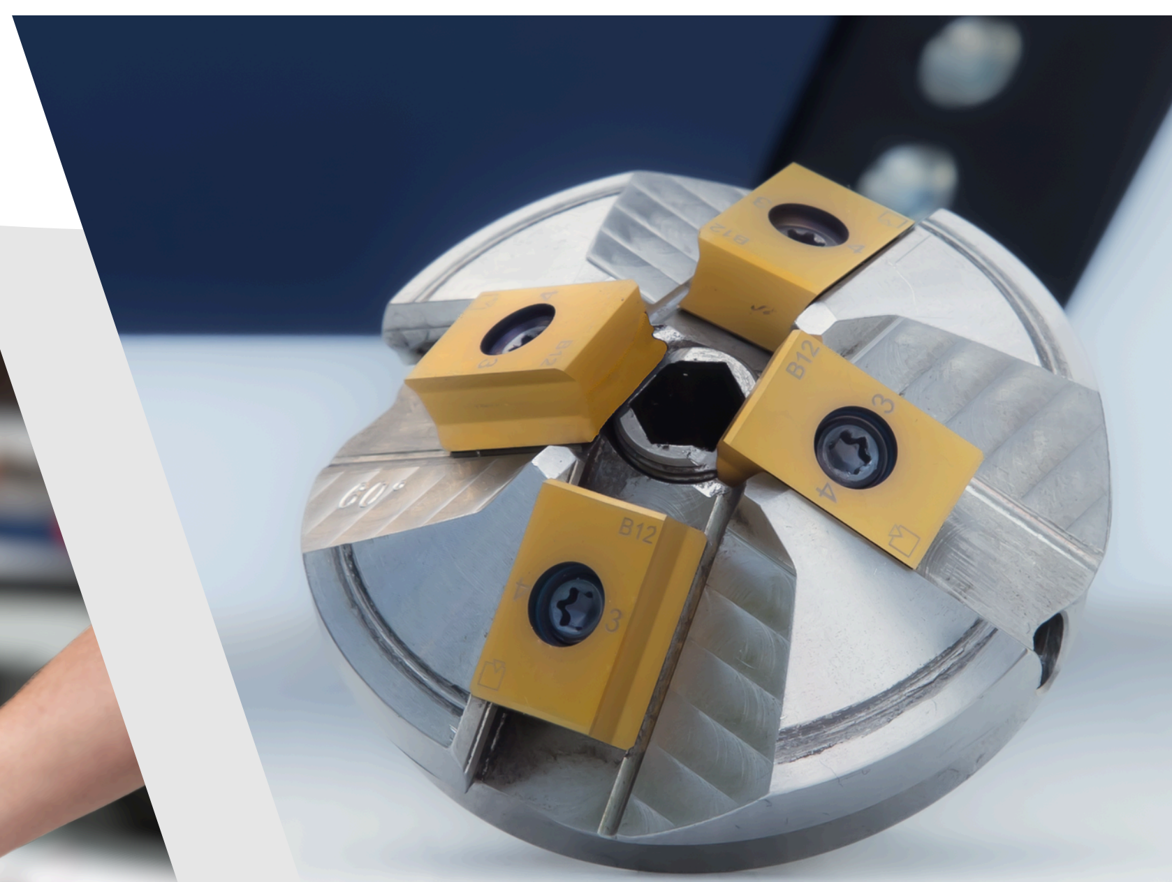
Fig. Milling head with indexable inserts
